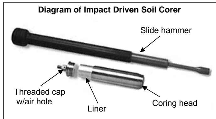
Figure 22-3. Diagram of Impact Driven Soil Corer
